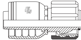
FPWK PRESSURE WASH FEMALE SWIVEL "K" TYPE
