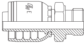
MBSPFF BSP FLAT FACE MALE
