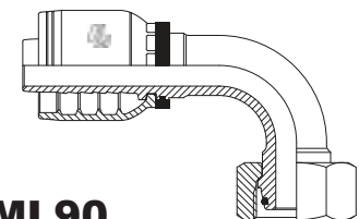
FML90 METRIC LIGHT FEMALE SWIVEL - 90° ELBOW (24° CONE SEAT) - DKOL
