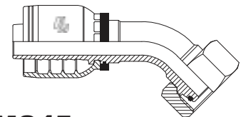
FMS45 METRIC HEAVY FEMALE SWIVEL - 45° ELBOW (24° CONE SEAT) - DKOS
