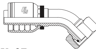
FML45 METRIC LIGHT FEMALE SWIVEL - 45° ELBOW (24° CONE SEAT) - DKOL
