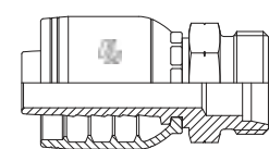
MML METRIC LIGHT MALE (24° CONE SEAT) - CEL
