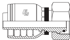
FML METRIC LIGHT FEMALE SWIVEL (24° CONE SEAT) - DKOL
