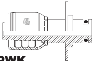
MPWK MALE SINGLE WASHER
