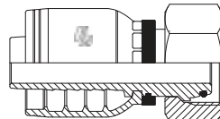
FMS METRIC HEAVY FEMALE SWIVEL (24° CONE SEAT) - DKOS
