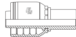
SP IMPERIAL STANDPIPE
