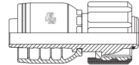
FPWW PRESSURE WASH FEMALE "W" TYPE
